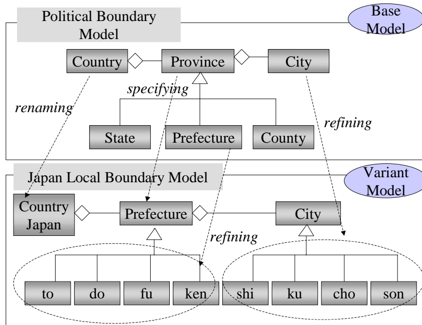
Figure F5- Example 4: Association Type "Base-Variant" (2)
