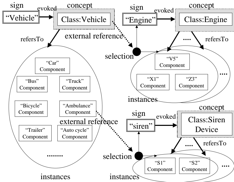
Figure E3- Registered Target connected with Selection
