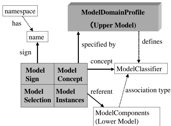
Figure E1- Basic Relationship of Registered Target Objects
