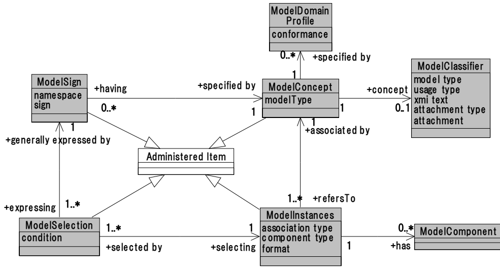
Figure 2- Registry Package in MMF Core
