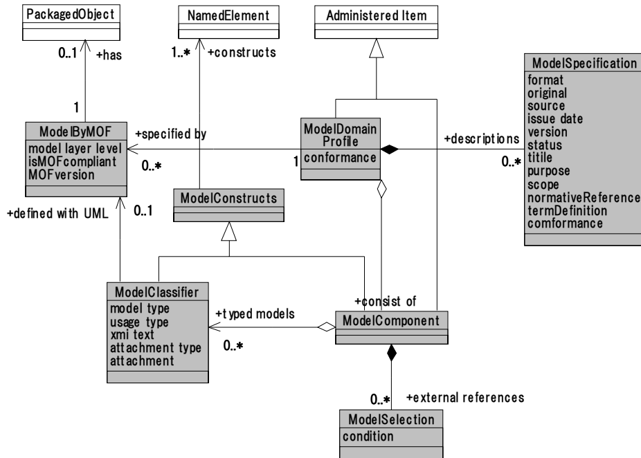
Figure 3- Target Package in MMF Core
