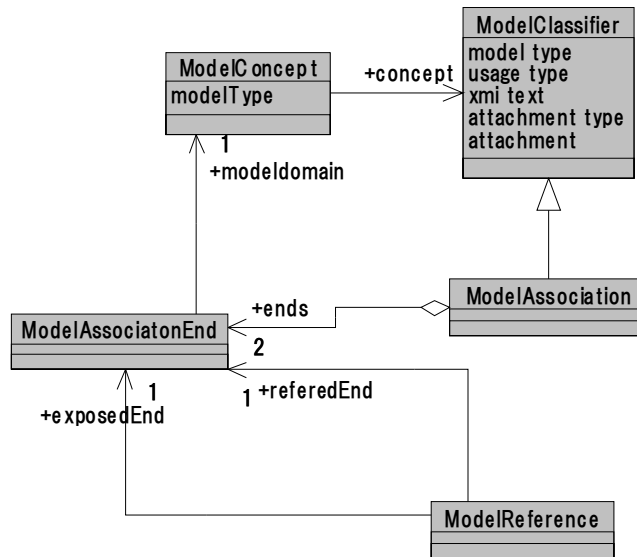
Figure 4- Relationship Package in MMF Core
