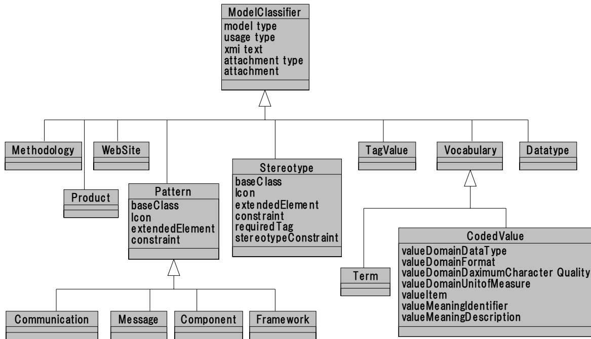
Figure C1- A Examples of ModelClassifier Package
