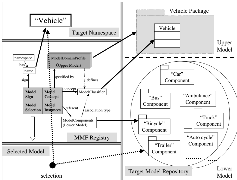
Figure E2- Registered Target Objects about “Vehicle”
