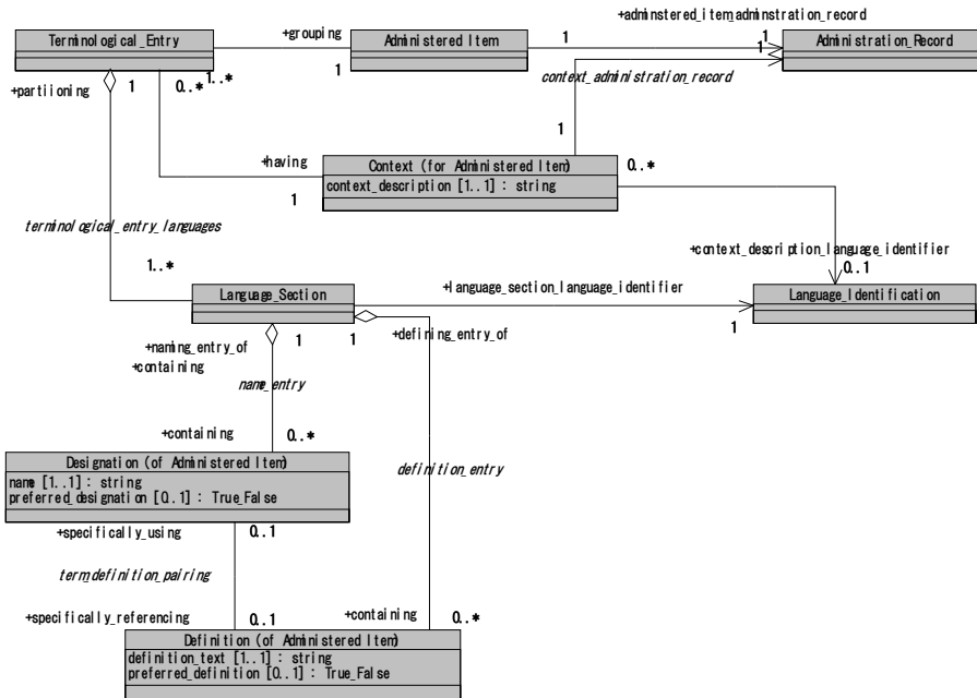
Figure A1- MDR Package (Administration and Identification)
