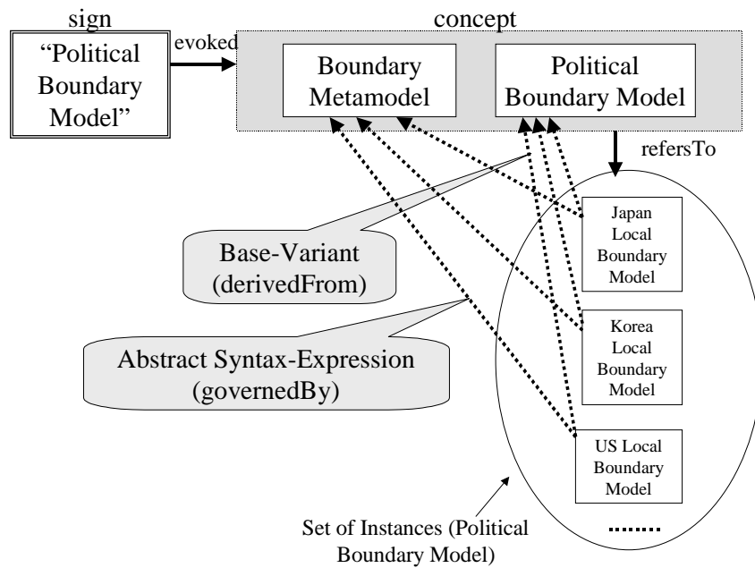
Figure F6- Example 5: Association Type “Abstract Syntax-Expression” (1)
