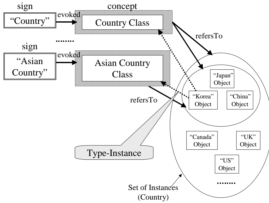
Figure F2- Example 2: Association Type "Type-Instance" (2)
