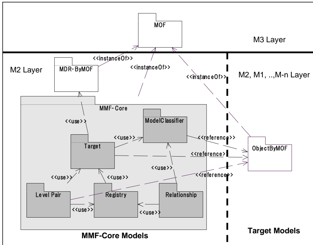
Figure 1- MMF-Core Packages and Target Models
