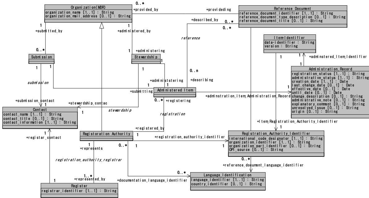
Figure A1- MDR Package (Administration and Identification)
