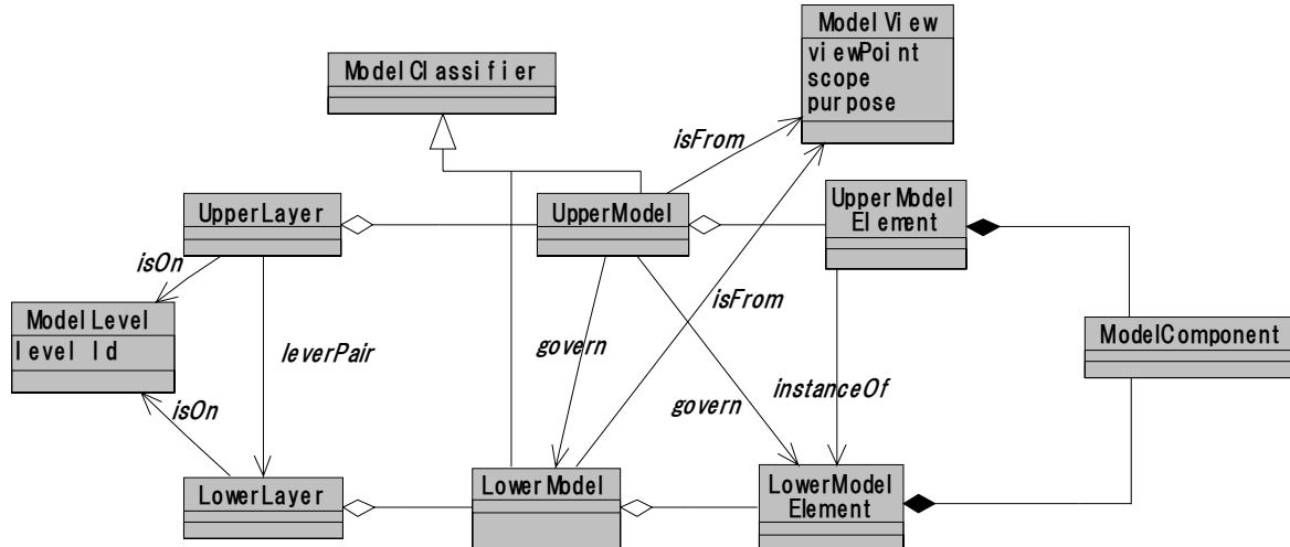
Figure D1- Level Pair Package
