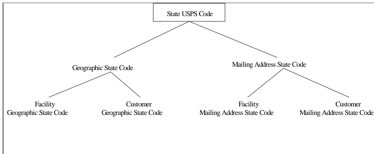
Figure 1 — Specialization/generalization hierarchy.
