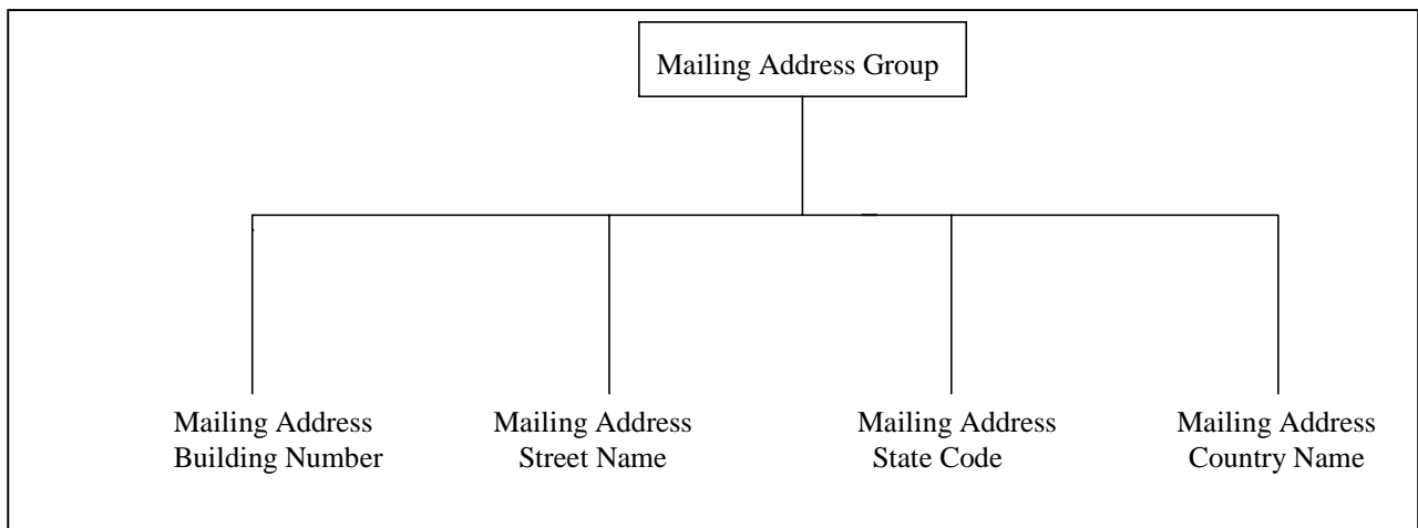
Figure 2 — Decomposition/aggregation example.
